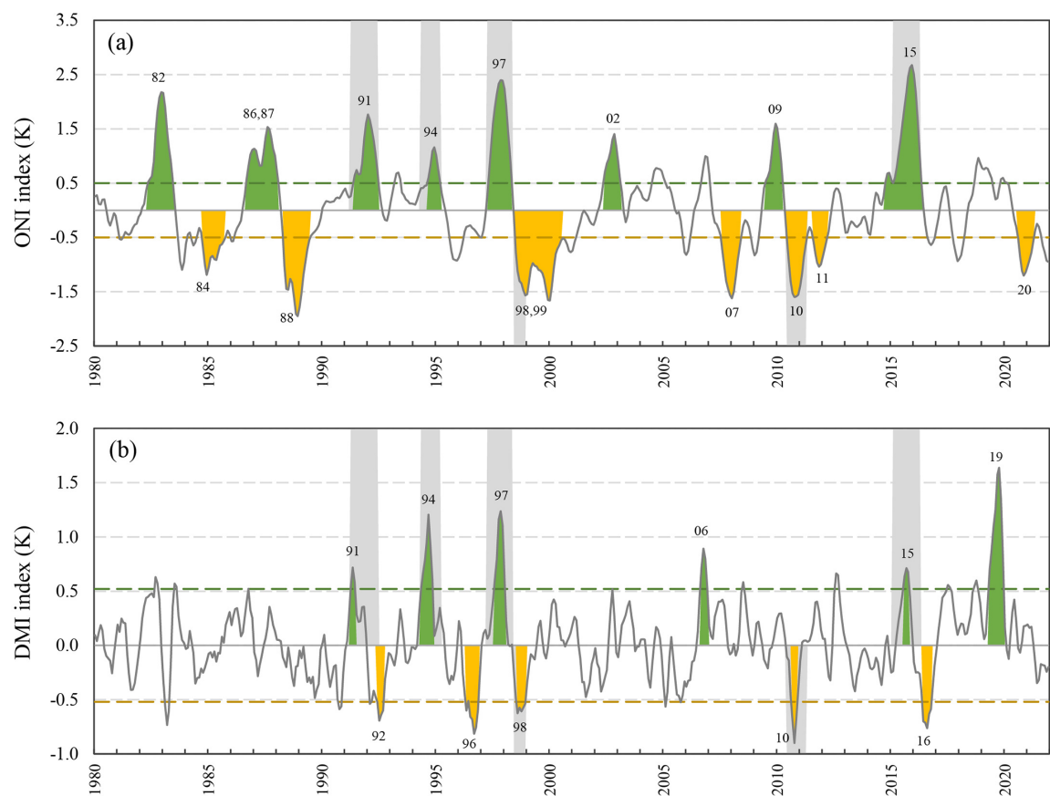
Figure 1. Time series of the Oceanic Niño Index (ONI) (a) and the Dipole Mode Index (DMI) (b) from 1980 to 2022. The positive phase events (El Niño and positive Indian Ocean Dipole, pIOD) are filled in green, and the negative phase events (La Niña and negative IOD, nIOD) are filled in yellow, and the events are also labeled with a two-digit year. The dashed green and dashed yellow lines represent the positive and negative thresholds for the El Niño–Southern Oscillation (ENSO) and IOD, respectively. The gray background indicates years with the simultaneous ENSO and IOD events.
