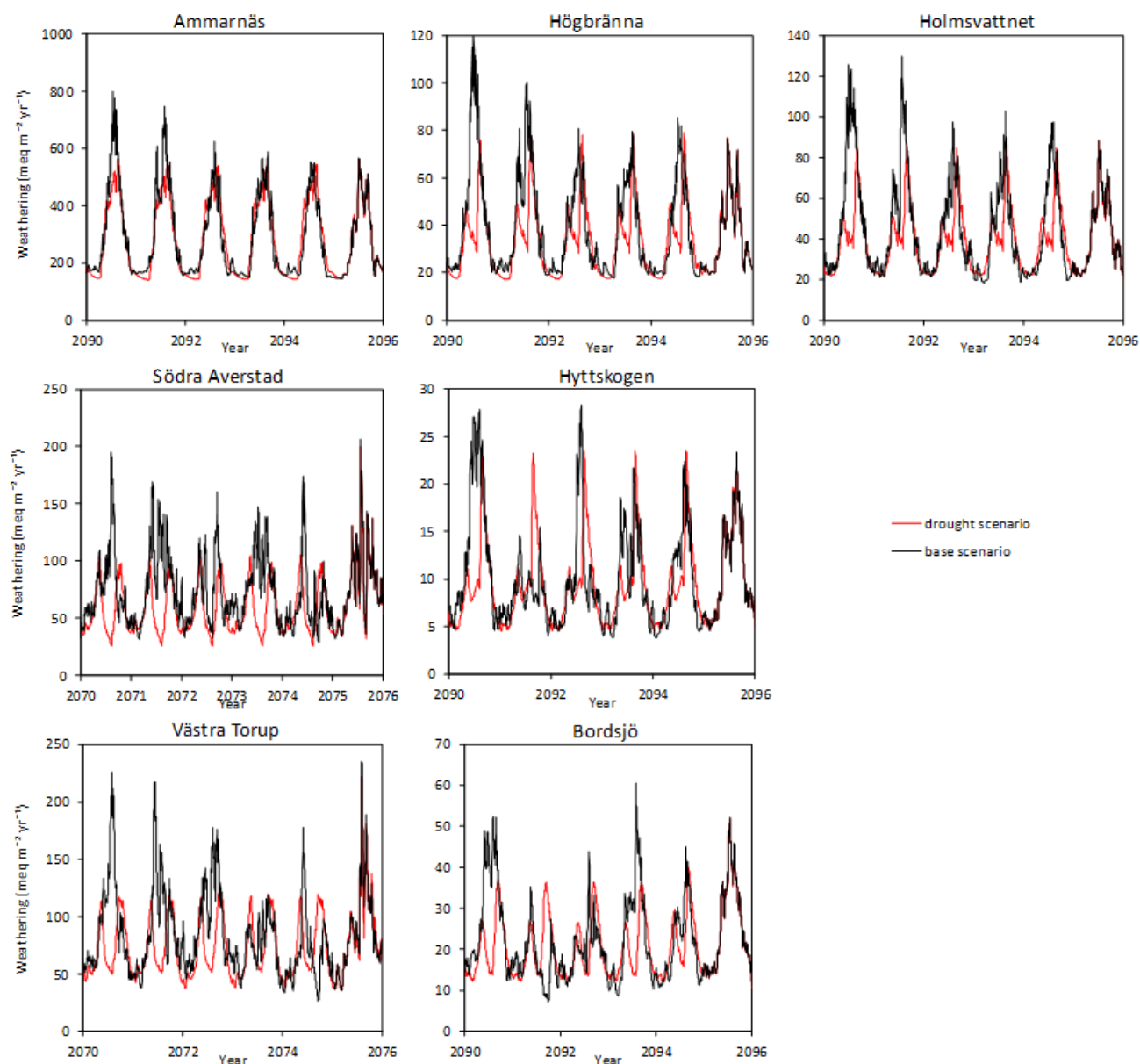
Figure 7. Weathering under the drought scenario (red) compared to the A1B scenario (black). The first year after the drought is also included. Weathering rates are the sum of Ca, Mg, K and Na for the humus layer and the upper 50 cm of mineral soil. For Södra Avestad and Västra Torup the drought occurs during the 5 years of 2070–2074, and for the other sites it occurs during 2090–2094. The upper three sites Ammannäs, Högränna and Holmsvattnet are situated in northern Sweden, and the sites in the middle and lower part of the figure lie in southern Sweden.
