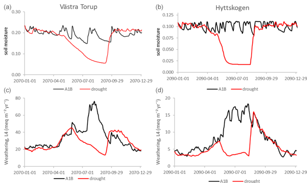
Figure 6. Different reactions of soil moisture (a, b) in sites with different texture during the first of the drought years: Västra Torup is less coarse textured than Hyttskogen and retains water for longer but also infiltrates water slower when precipitation resumes. This also affects the reaction of weathering rates of base cations to droughts (c, d).
