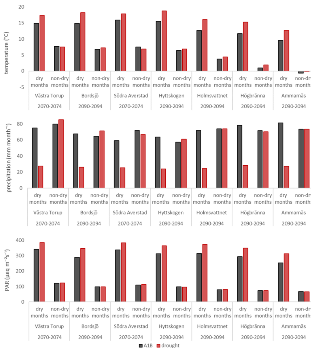
Figure 3. Monthly average temperature, precipitation and PAR (photosynthetic active radiation) during the A1B scenario (black) and the extreme drought scenario (red) for months with drought (April to July) and months without drought (August to March). For Södra Averstad and Västra Torup, the drought occurs during the 5 years of 2070–2074, and for the other sites it occurs during 2090–2094. The sites are ordered from south to north in the figure, with the southernmost (Västra Torup) at the left and the northernmost (Ammarnäs) at the right.
