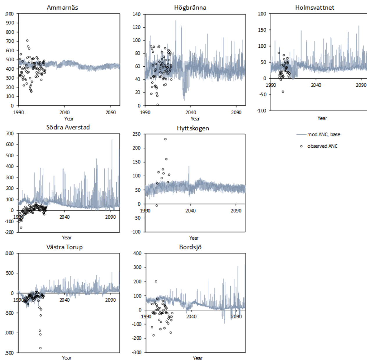
Figure A1. Development of soil water chemistry – daily modelled ANC from 1990 to 2100 and observed values three times a year, from lysimeters at 50 cm depth, in the seven sites.
